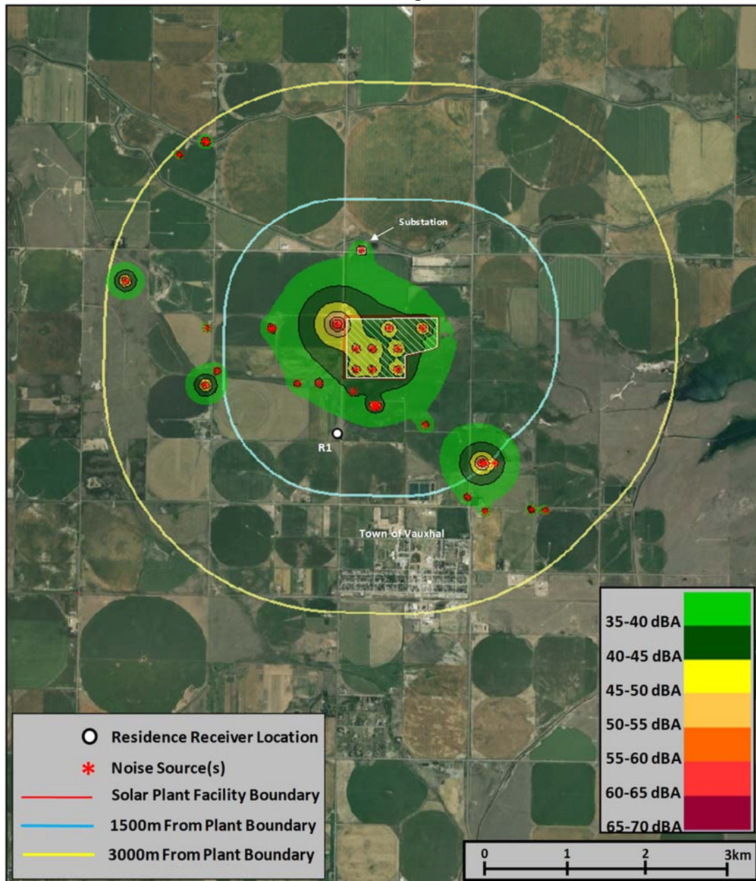
Figure 3 Facility Contribution Noise Contour Solar Krafte Prairie Sunlight III Solar Plant
